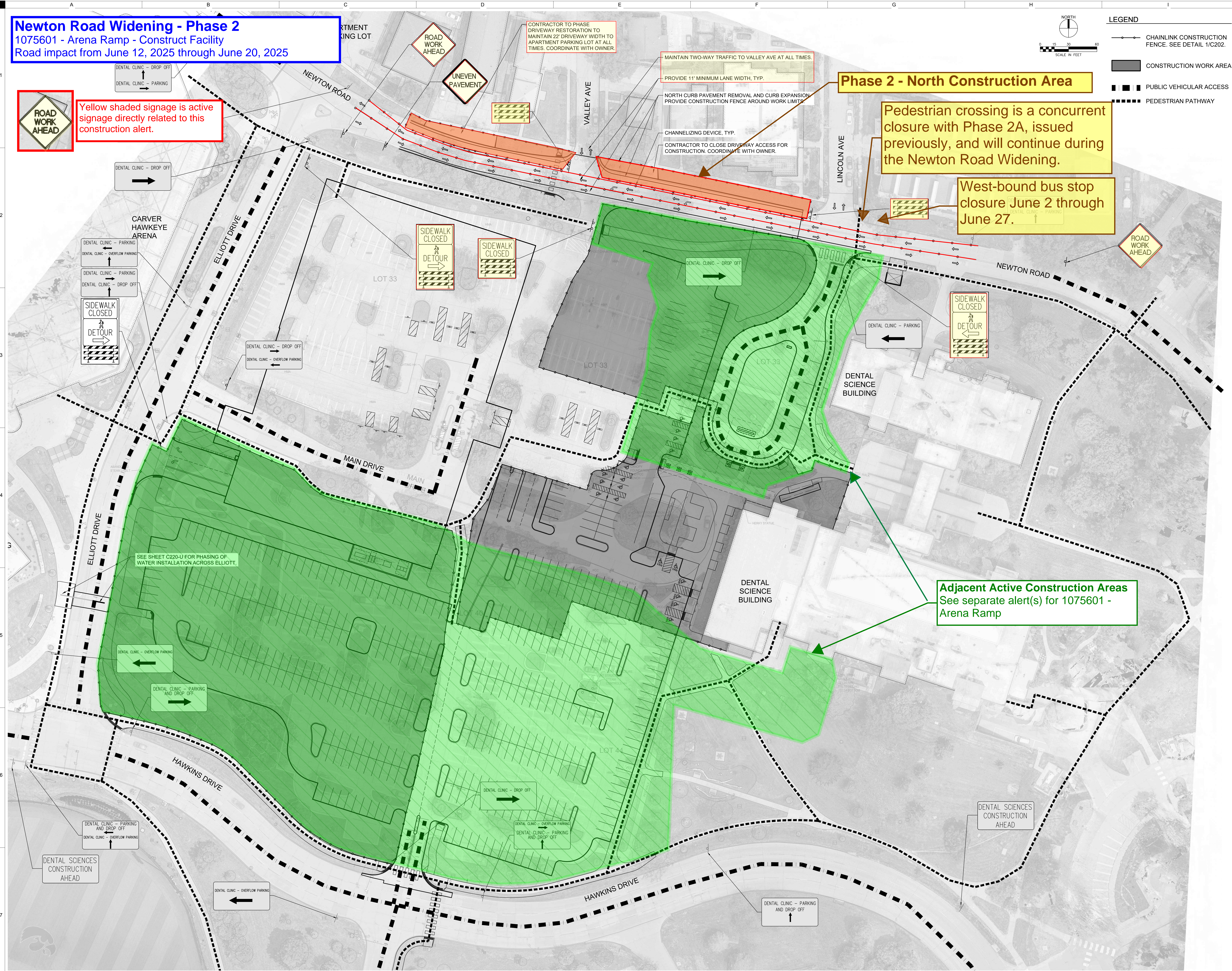
TRAFFIC CONTROL - PHASE 2B
