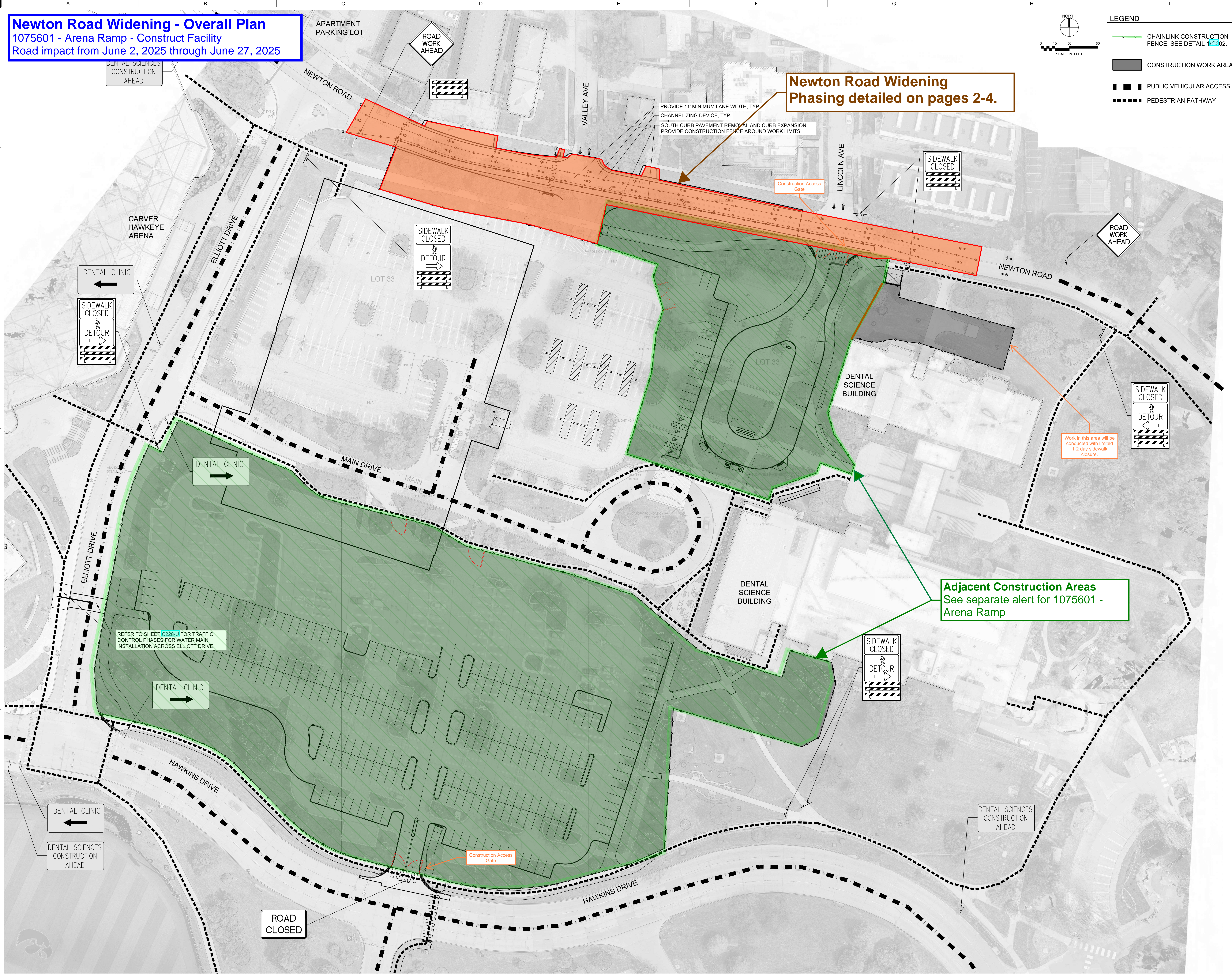
TRAFFIC CONTROL - PHASE 2A
