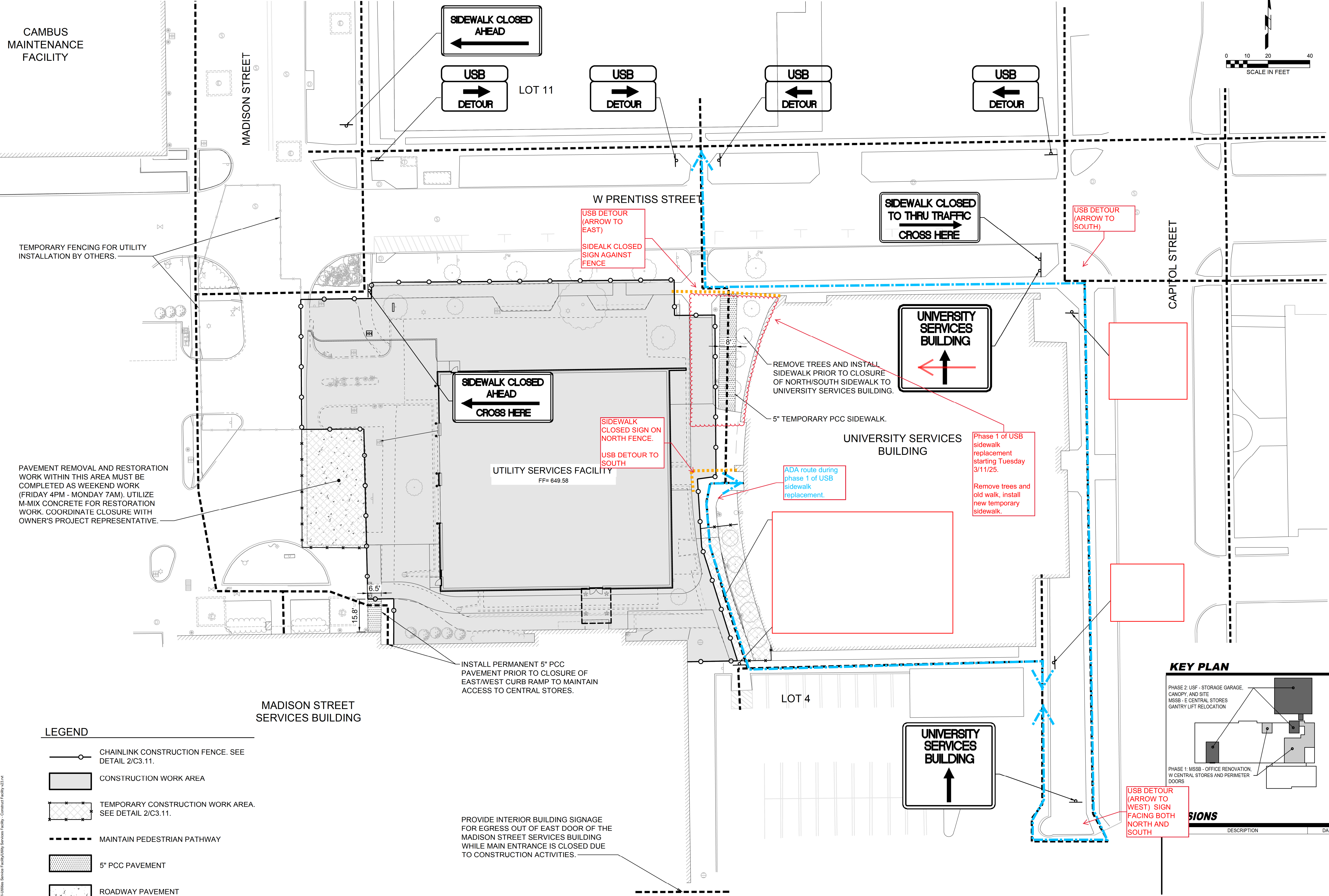
PLAN - TRAFFIC CONTROL
